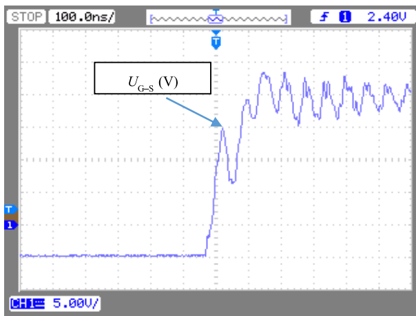
Fig. 12: Obtained switching on process detail at U_{IN} = 1000 V - gate-source voltage measured directly on power transistor (V).
