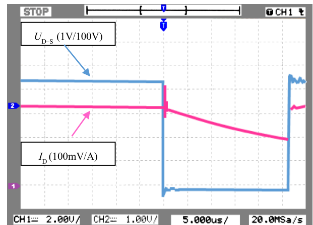
Fig. 9: Obtained one-pulse switching process at U_{IN} = 1000 V, drain-source voltage 1:100 (V) - blue curve, drain current 100 mV/A (V) - violet curve.
